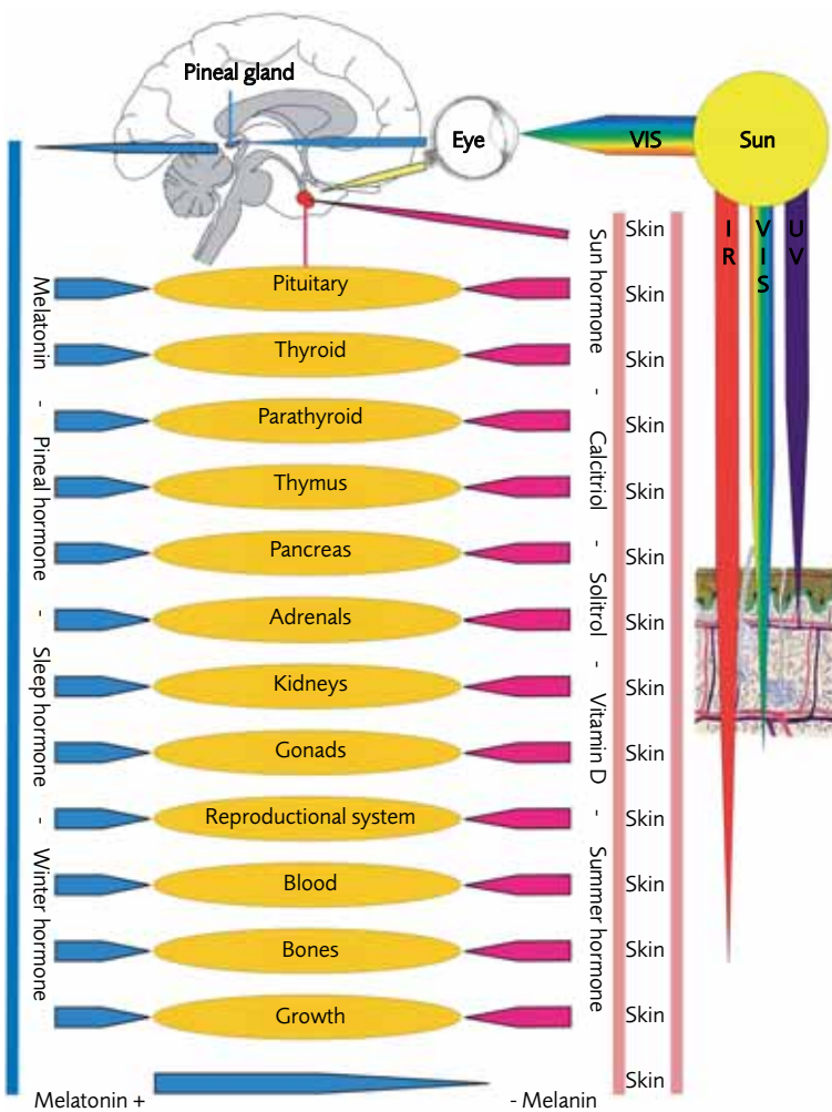
The effect of light on human skin, the human eye and the human hormone system.
