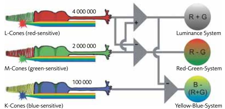
Principle behind the switching of colour-sensitive receptors in the human retina.
