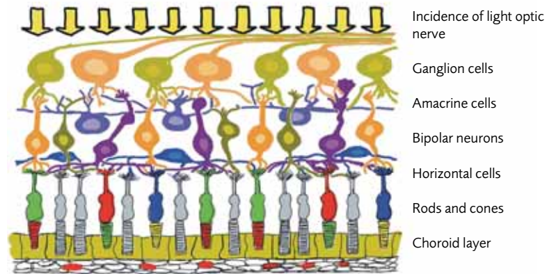
Light-processing layers of the retina.
