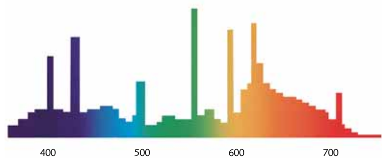
Spectrum of discharge lamps.
