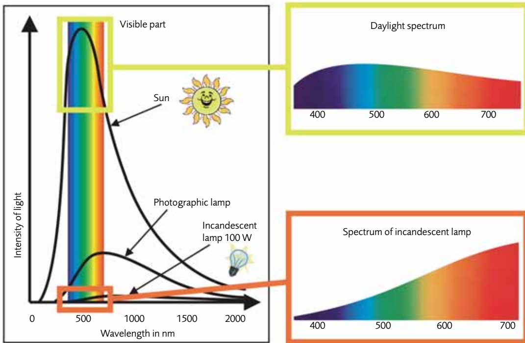
Spectrum of a glowing black body at the temperatures of a normal incandescent lamp, a photographer's lamp and the sun.
